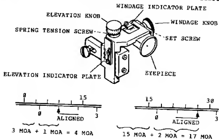
Figure 2-13. Rear sight adjustment.
